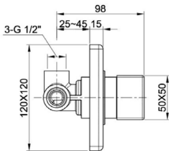
AP5005 MISCELATORE DOCCIA INCASSO CONCEALED SHOWER MIXER BRAUSEMISCHER UP
